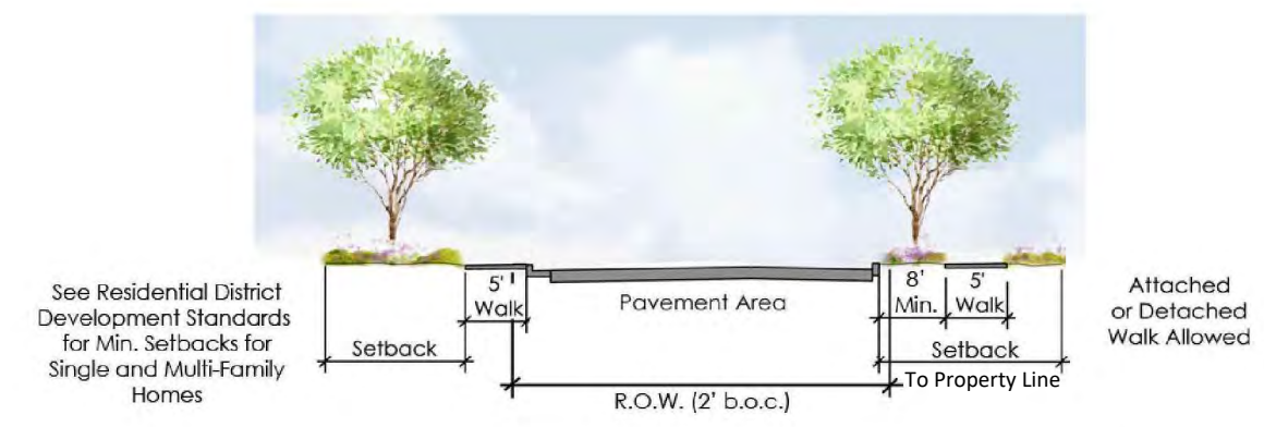
==== Local Street Section
